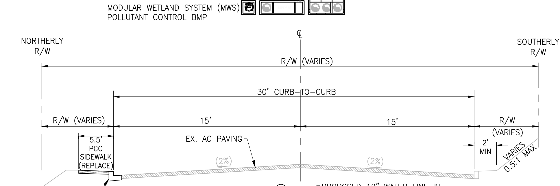
SECTION - CROUCH STREET SOUTH OF PROJECT PROPERTY SCALE: N.T.S.
