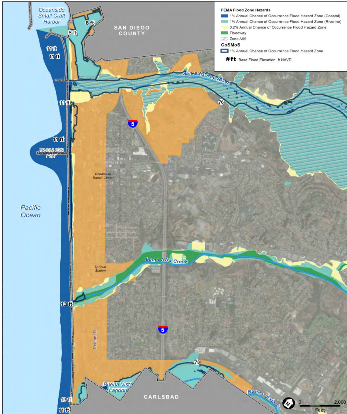
Figure A-2 FEMA and CoSMoS Flood Inundation Areas (Coastal Zone shown in orange)
